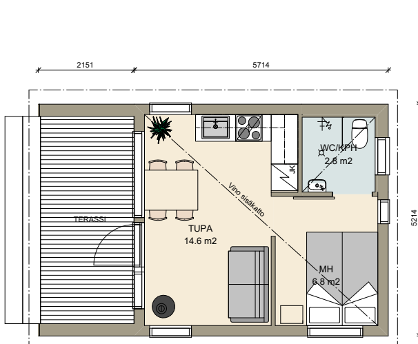
tupa, 1 mh, wc
